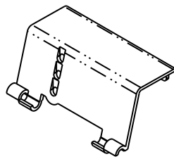
ITEM 8 FM-3 - LOWER FRONT COVER
