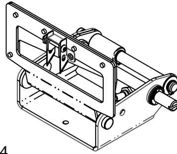
ITEM 44 FM-26-XXX-EZ ROCKER BLADE W/TAB CUTTER SUB-ASSY
