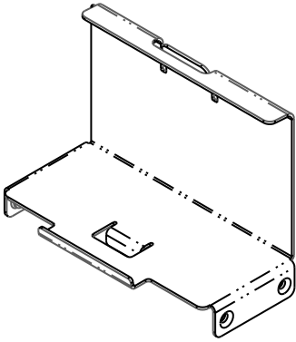
ITEM 43 TS33-032-01 - SAFETY BAFFLE (4 PIECES OF ST-1949, SCREW-#10-24 x 3/8" LG)
