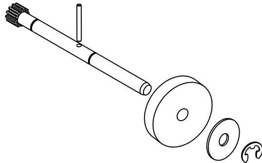
ITEM 46 FM-304-K FEED WHEEL CONVERSION KIT
